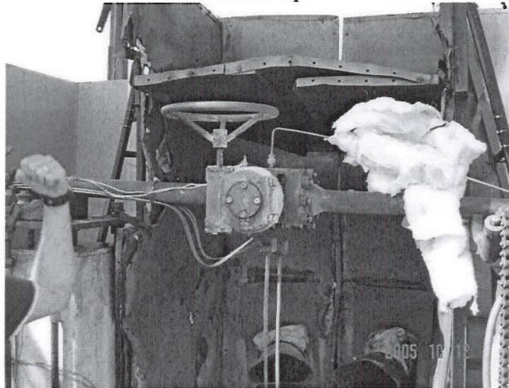
Valve after completion of Burn
