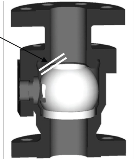
Lock-Up Gap
