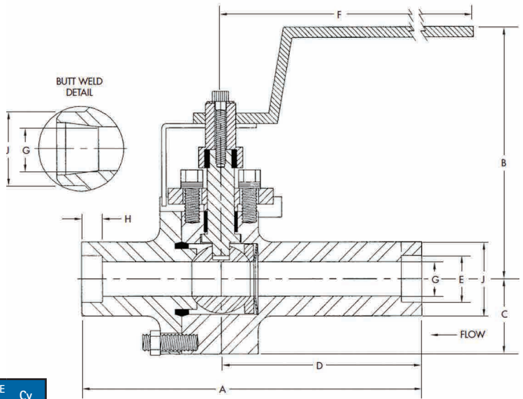
Note: Drawing represents 1/2" and 3/4" valves only.
