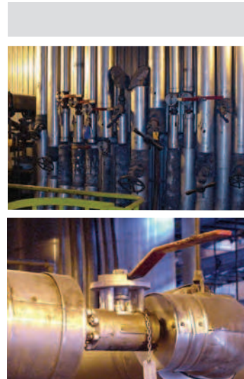
Pictured above: Main steam hot and cold reheat drain and vent valves. Steam is returned to the turbine in the hot reheat line at 1000°F (538°C), 600 psi (41 bar). The drain valves are used to heat the steam lines during start-up and discharge into condenser.
